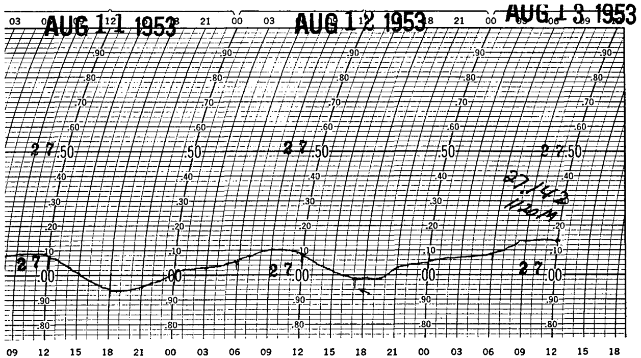
FIGURE 2.—Microbarogram, St. George, Utah, August 11–13, 1953. The arrow points to the pressure drop trace of the dust devil, August 12, 1953. Similar vertical marks at other points on the trace are time checks.
